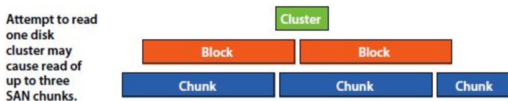
Figure 2.33: Unaligned partitions
