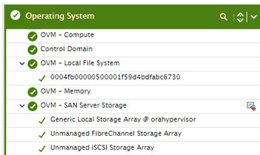
Figure 2.24: The tests mapped to the Operating System layer
