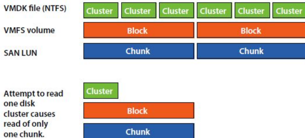
Figure 2.34: Aligned partitions
