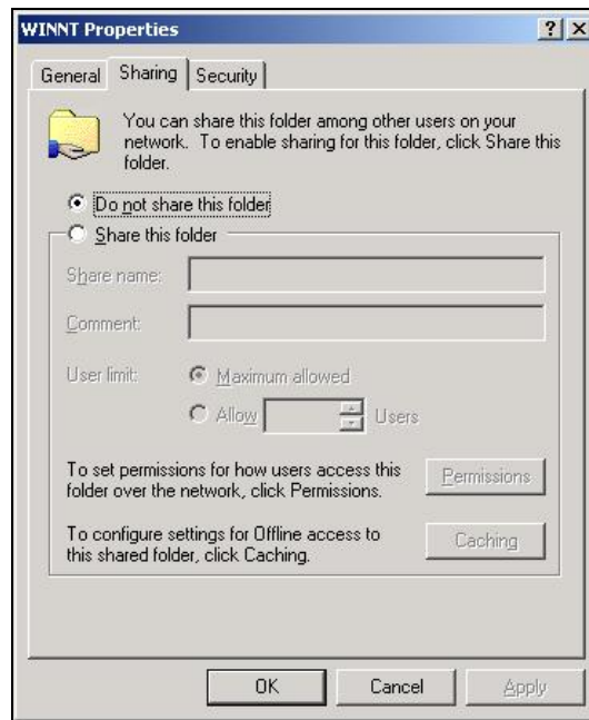
Figure 2.1: The ADMIN$ share does not exist
