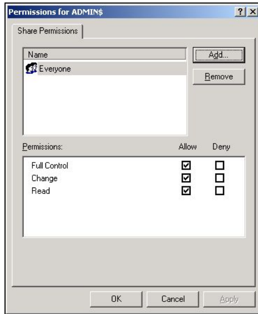
Figure 2.4: Clicking the Add button
