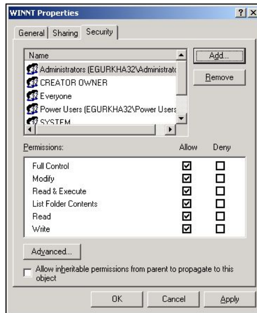
Figure 2.7: Defining the Security settings for the ADMIN$ share
