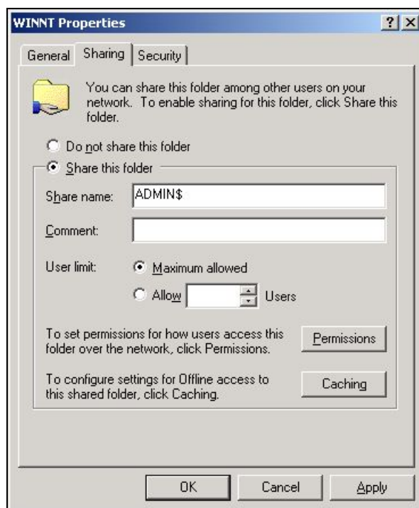
Figure 2.3: Creating the ADMIN$ share
