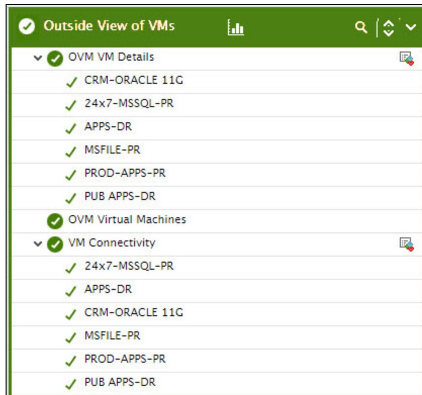
Figure 2.29: The tests mapped to the Outside View of VMs layer
