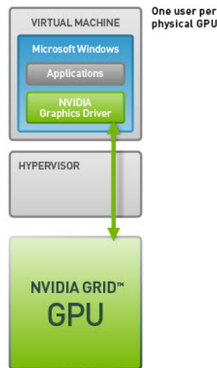
Figure 4.8: Dedicated GPU Technology
