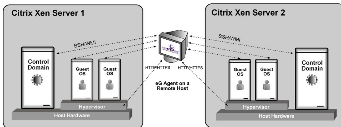
Figure 2.2: Monitoring Citrix XenServers in an agentless manner
