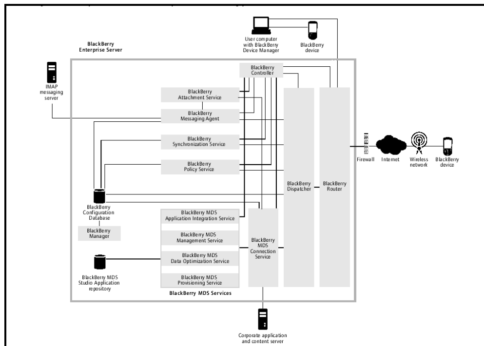
Figure 1.1: Architecture of the BlackBerry Enterprise Server
