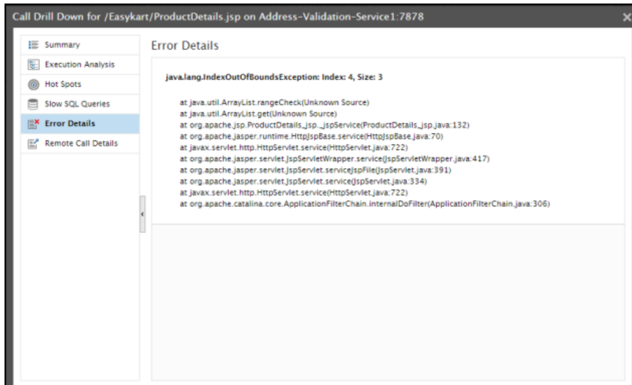
Figure 3.17: Error details
