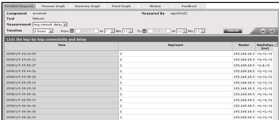
Figure 2.11: Detailed diagnosis of the Average delay measure listing the hop-by-hop connectivity and delay
