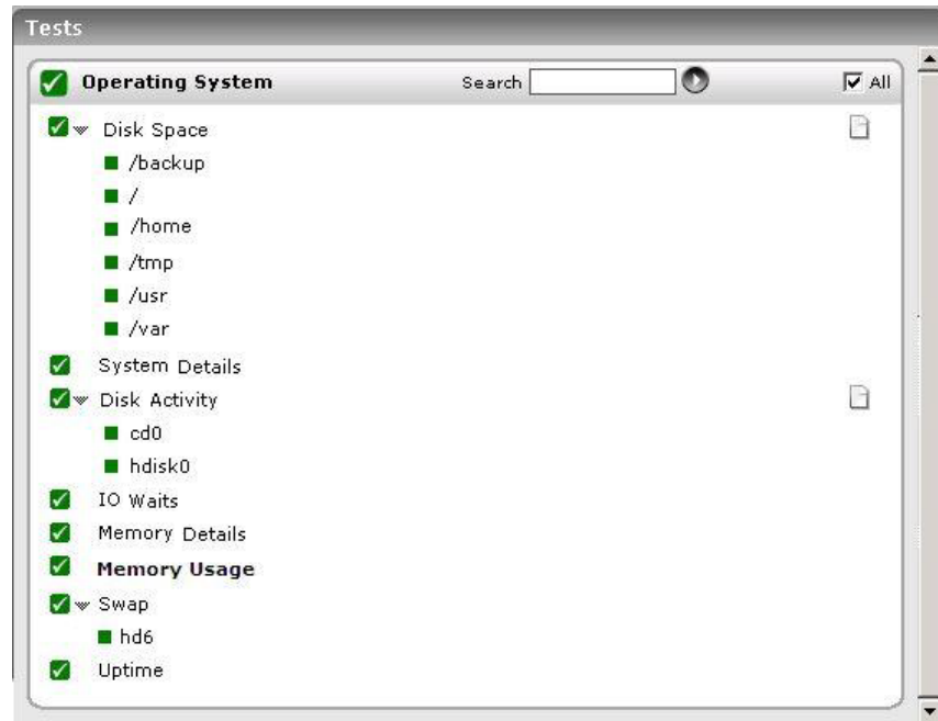
Figure 2.21: Tests that map to the Operating System layer of a Solaris server
