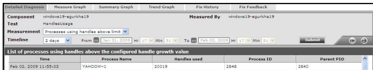
Figure 3. 5: The detailed diagnosis of the Processes using handles above limit measure
