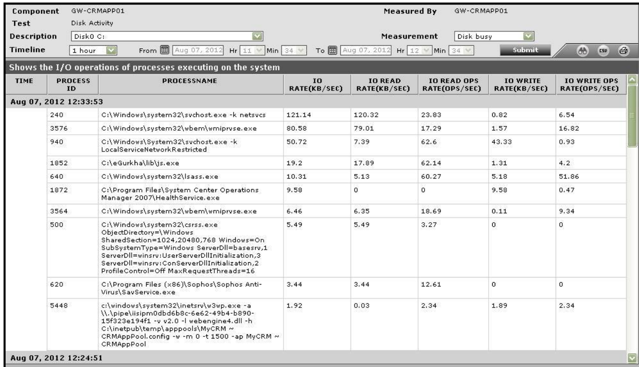
Figure 3.3: The detailed diagnosis of the Disk Activity test
