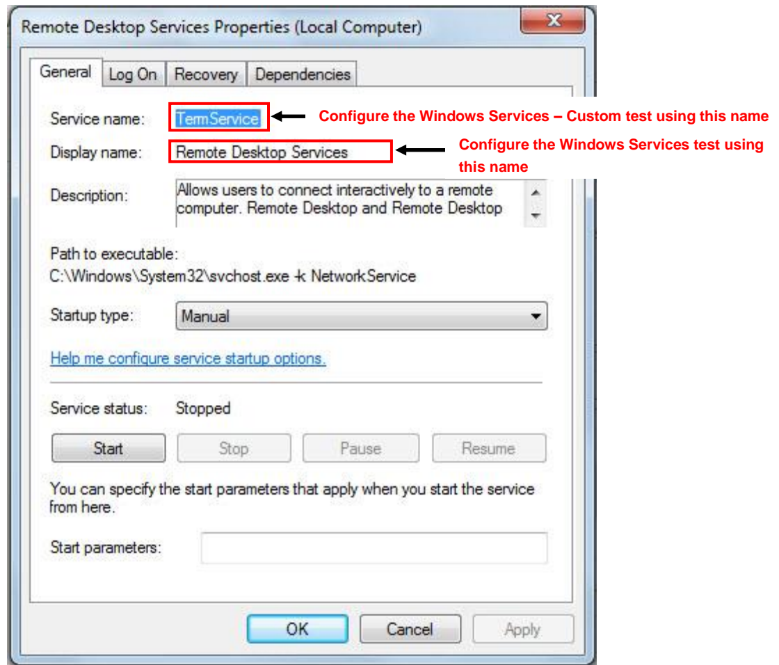
Figure 3.28: The Service Properties window
