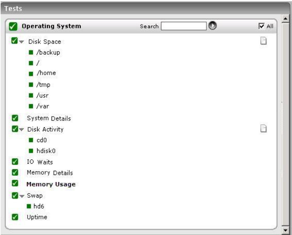
Figure 2.25: Tests that map to the Operating System layer of an AIX server
