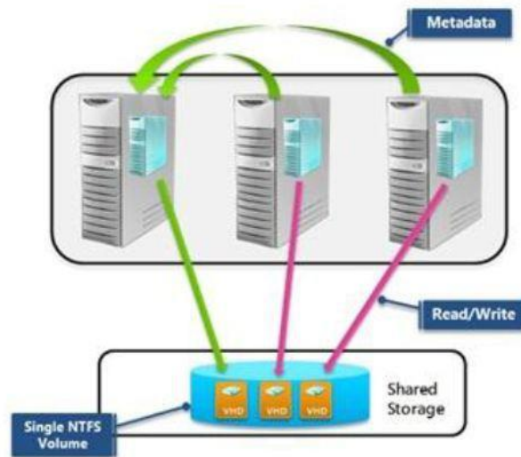
Figure 3.19: How the Cluster Shared Volume works?
